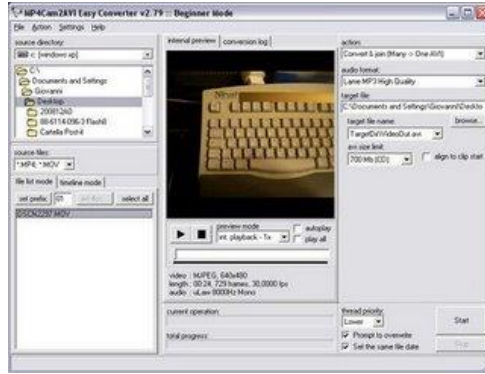
MP4Cam2AVI
